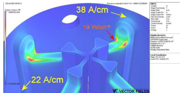
Figure 4: 3D view of the power deposition
