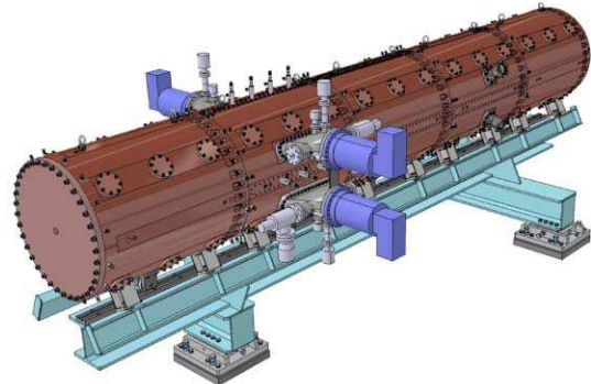
Figure 7 : Artistic view of the final SPIRAL2 RFQ
