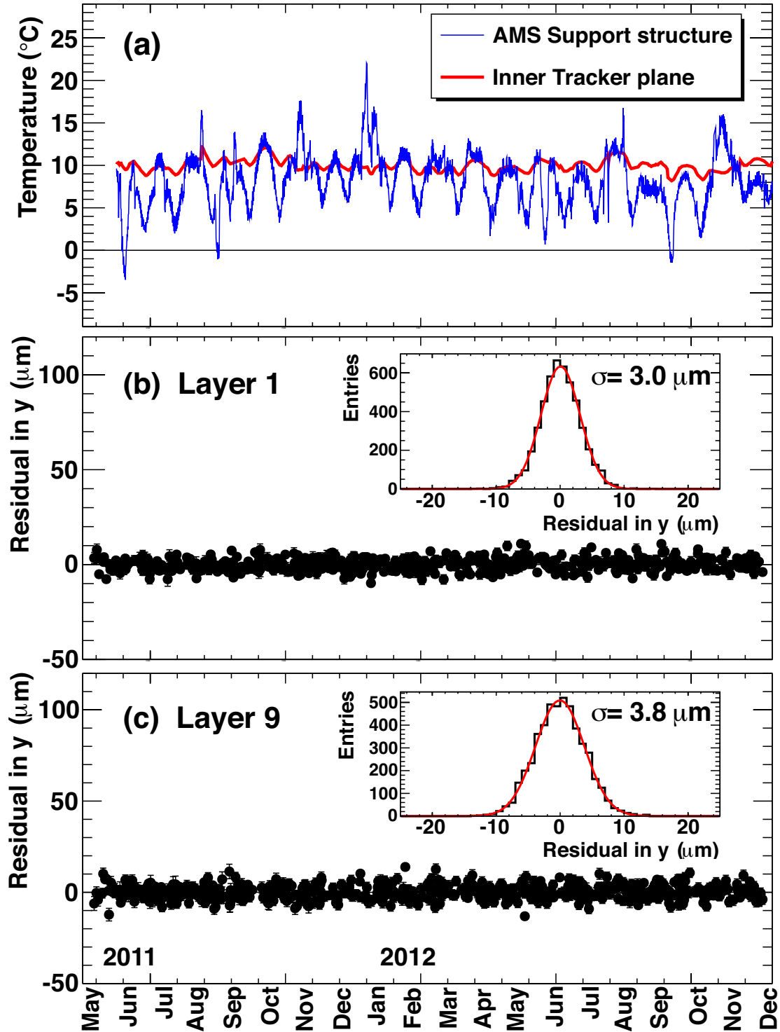
FIG. 2. Stability of the alignment of Tracker planes over more than 18 months of operation. (a) The temperature of the AMS support structure varies by 25^\circ\text{C} , whereas the temperature of the inner Tracker planes remains within 1^\circ\text{C} . As shown in (b), (c) and their inserts, the position of the outer planes 1 and 9, respectively, aligned using cosmic ray protons results in the precise tracing of their thermal movement over more than 18 months to a stability of 3 \mu\text{m} .
