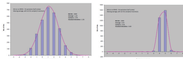
Figure 4: Stability studies of mechanical assembly with piezo-movers supporting the third IP-BPM.
