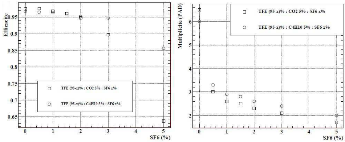
Figure 2: GRPC efficiency ( left ) and multiplicity ( right ) as a function of the proportion of \text{SF}_6 electron quencher. Measurements have been done with 7.1 kV high voltage and 135 fC signal threshold detection. Two UV-photon quenchers have been tested : isobutane and \text{CO}_2 .
