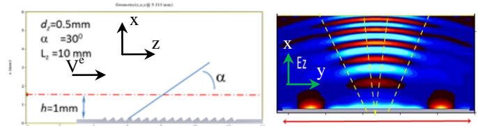
Figure 1: (a) Full 3D Numerical model of a broadband cSP radiator observed using PiC code MAGIC; (b) Contour plot of E_z field component generated by the fs-bunch ( x - y plane) at the middle of the grating.
