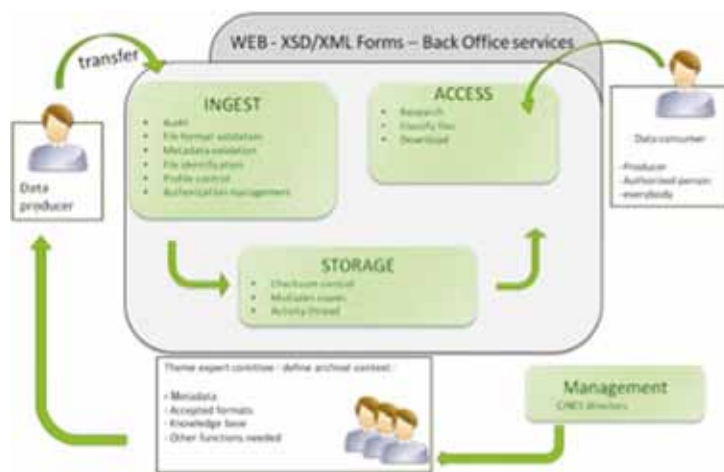
Figure 3. ISAAC system workflow.
