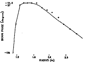
Fig 7b : Phase law with \partial W / \partial B = 0
