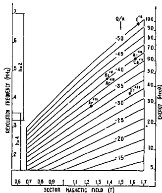
Figure 2 : Basic beam characteristics
