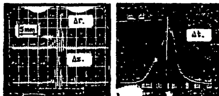
a H and V beam profiles at the \alpha -spectrometer b At given by X-ray bunch length monitor
