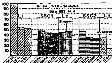
Fig.2 : Characteristics of a Kr beam : a) energy spread = 1.2 \cdot 10^{-4} , FW : 0.3\% FWHM b) phase spread = 6.7 ns FW, 2 ns FWHM ( 1 \text{ ns} = 3^\circ ) c) H and V emittances : not well matched in H plane. d) transmission efficiency all along the machine.
