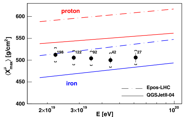
FIG. 8 (color online). \langle X_{\text{max}}^\mu \rangle as a function of energy. The predictions of different hadronic models for protons and iron are shown. Numbers indicate the number of events in each energy bin, and brackets represent the systematic uncertainty.
