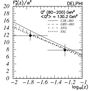
Fig. 6. LEP II data. The F_2^e measured for Q^2 \in (80, 200) \text{GeV}^2 . For each bin the total uncertainty is plotted (the data is corrected for the absence of radiation in the theoretical prediction).
