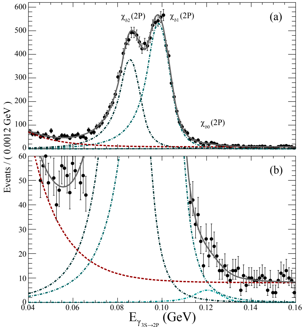
FIG. 5: (a) Fit to the soft photon energy E_{3S \rightarrow 2P} in the 3S \rightarrow 2P \rightarrow 1S cascade with individual signal (signal corresponds to the small bump) and background (dash) components for the calorimeter-based analysis. (b) A zoomed-in view of the \chi_{b0}(2P) peak on the same energy scale. Discussion of the significance of the J = 0 peak is contained in Section IV C.
