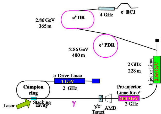
Figure 1: CLIC Injector Complex with Compton Ring
