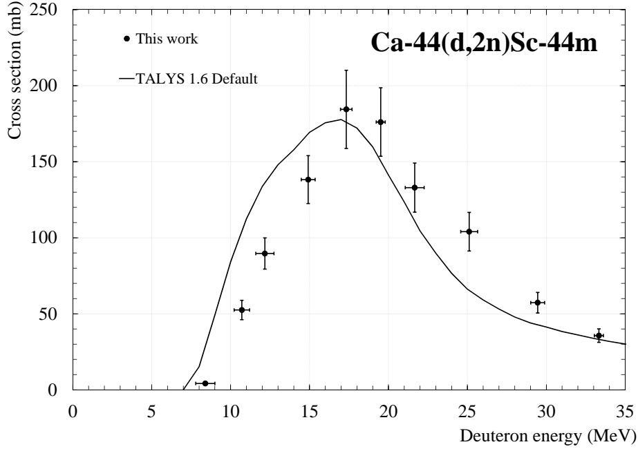
Figure 3: Excitation function for the Ca-44(d,2n)Sc-44m reaction
