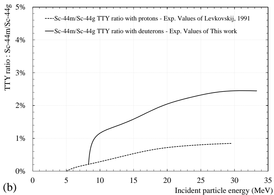
Figure 10: Experimental Sc-44m/Sc-44g cross section (a) and calculated TTY (b) ratios using protons and deuterons as projectiles
