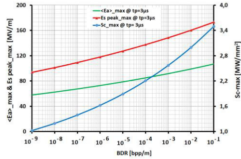
Figure 5: Dependence of the expected BDR versus average accelerating gradient, surface electric field and the modified Poynting vector for the prototype.
