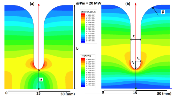
Figure 3: Distribution of (a) electric field and (b) modified Poynting vector in the regular cell.
