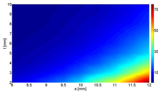
Figure 2: The optimization quantity \eta in the iris region.
