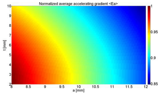
Figure 1: Normalized average accelerating gradient as function of the iris radius and thickness.
