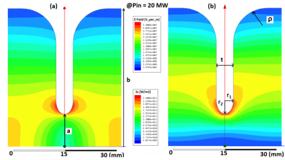
Figure 3: Distribution of (a) electric field and (b) modified Poynting vector in the regular cell.
