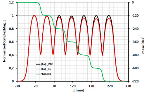
Figure 4: Amplitude and phase of the accelerating gradient along the prototype's axis.
