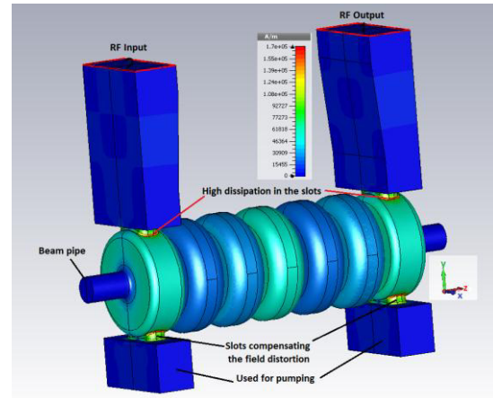
Figure 6: Surface magnetic field distribution for an input power of 20 MW (peak value).
