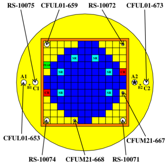
Fig. 2. Schematic view of the CR0 \downarrow configuration. The black star shows the position of the external neutron source (Am-Be). Control rods (CR) are in red.
