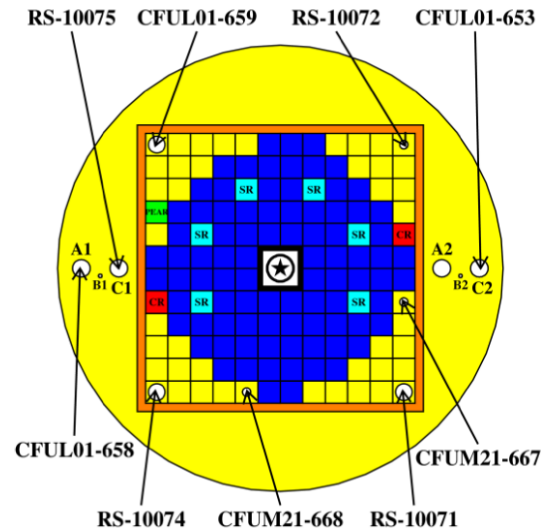
Fig. 3. Schematic view of the SC1 \downarrow configuration. The black star shows the position of the external neutron source (GENEPI-3C). Control rods (CR) are in red.
