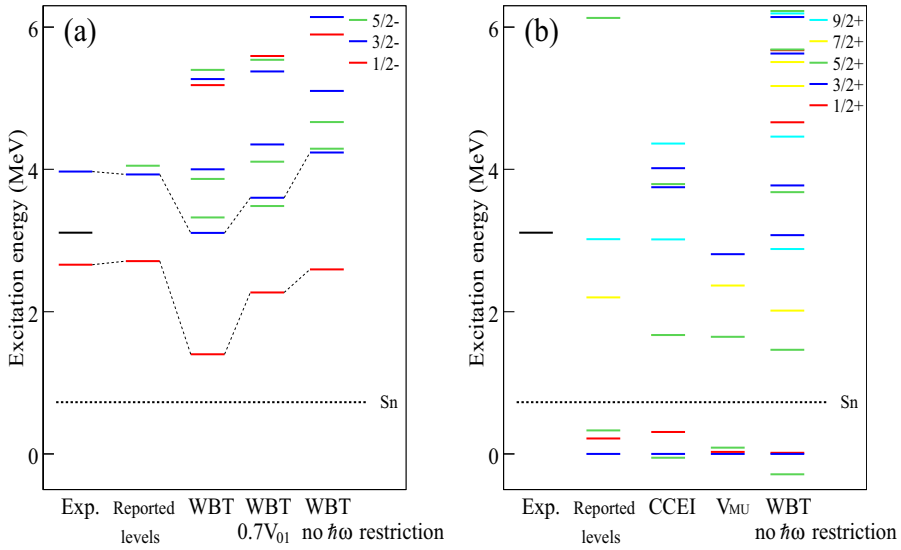
Figure 1. Negative (a) and positive (b) parity states in ^{17}\text{C} . "Exp." refers to the states observed in this study. For others see the text.
