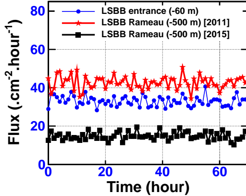
Figure 4. Comparison of the detected particle flux with (2015) and without (2011) ventilation system.
