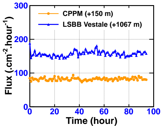
Figure 3. Detected particle flux for the atmospheric sites.
