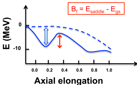
Figure 1. Potential energy of the nucleus as a function of axial deformation. The dashed line shows the liquid drop prediction for ^{264}\text{Hs} ( Z=108 ). The solid line shows the effect of shell corrections on the potential energy.
