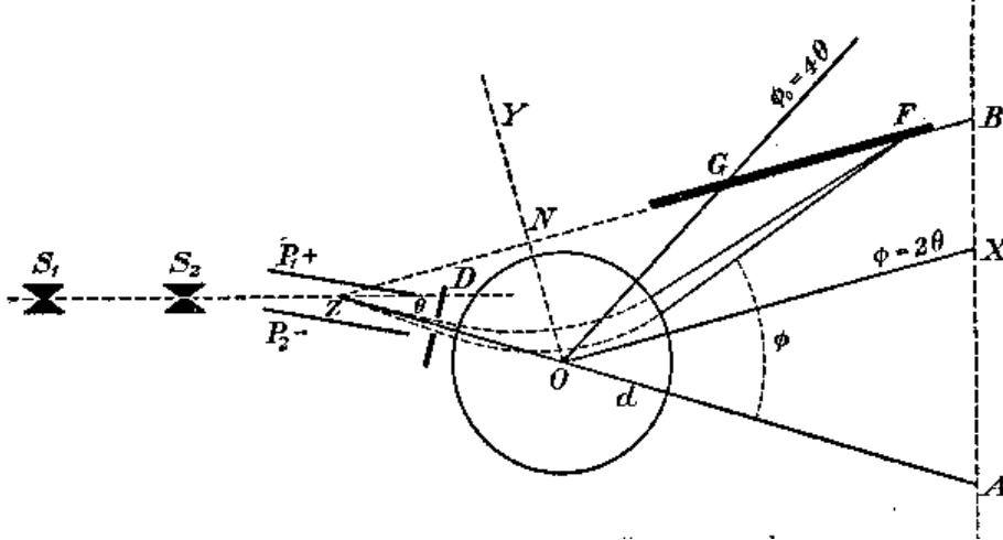
Figure 2: Diagram of Aston's first mass spectrograph (1919). The narrow slits S_1 and S_2 define a beam with very small divergence. They are deflected and dispersed by the electric field between P_1 and P_2 . The diaphragm D selects ions in a small window in energy which enter the magnetic field and are refocused at F on the photographic plate GF . From Ref. [1].
