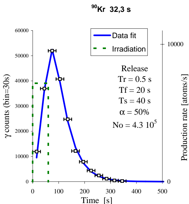
FIG. 2. (Color) Time distribution for release and transport of ^{90}\text{Kr} observed at cold finger. The solid line corresponds to a fit (see text).
