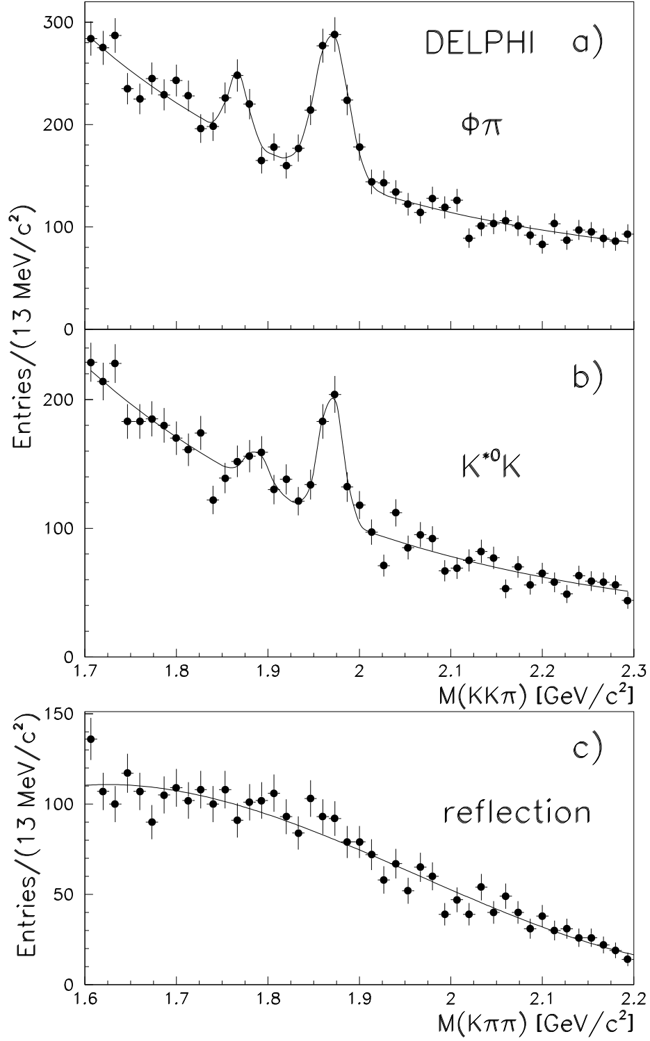
Figure 5: D_s h analysis: The invariant mass distribution for the inclusive D_s^+ samples for the a) D_s^+ \rightarrow \phi\pi^+ and b) D_s^+ \rightarrow \bar{K}^{*0}K^+ decay channels; c) shows the invariant mass distribution for the combinations shown in b) if the K^+ is assigned the \pi^+ mass. The curves show the fits described in the text.
