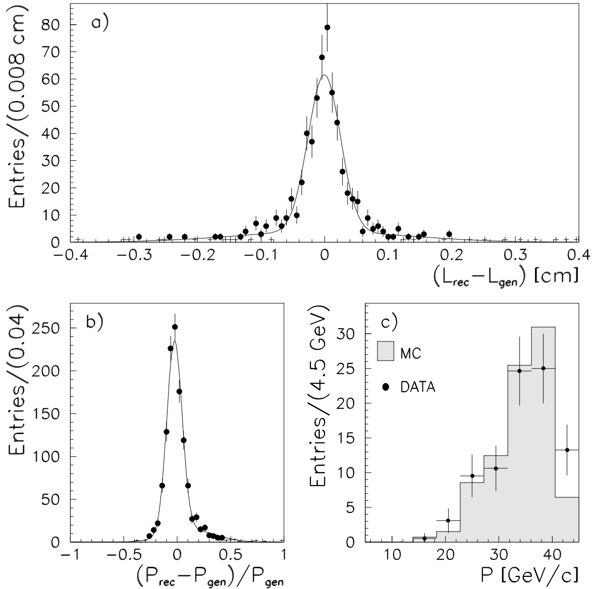
Figure 3: D_s \ell analysis: \overline{B}_s^0 decay length (a) and momentum (b) resolution for the \phi\pi^+ and \overline{K}^{*0}K^+ decay modes of the D_s^+ . The curves show the fits described in the text. c) Comparison between the momentum distribution from simulated events and that estimated from real data by subtracting the momentum distribution of events in the D_s^+ side bands from that of the events in the signal region.
