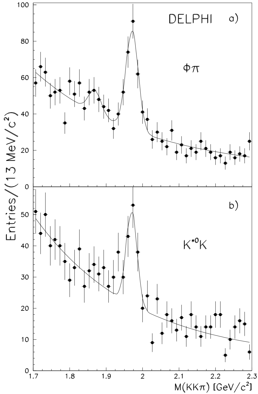
Figure 8: D_s h analysis: KK\pi invariant mass distributions for the D_s^\pm - h^\mp samples for a) D_s^+ \rightarrow \phi\pi^+ and b) D_s^+ \rightarrow \bar{K}^{*0}K^+ . The curves show the fits described in the text.
