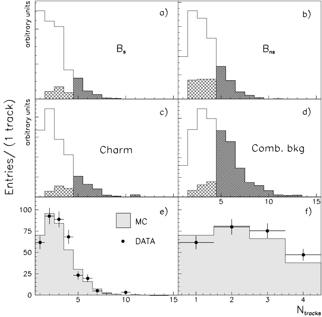
Figure 7: D_s h analysis: a) - d) Charged multiplicity distributions for tracks accompanying D_s^+ mesons and coming from different sources. The lightly hatched areas show the effect of removing identified “right-sign” kaons. The heavily hatched areas show the effect of the multiplicity cut. The next two figures show the charged particle multiplicity distributions after combinatorial background subtraction in the mass interval \pm 2\sigma around the measured D_s^+ mass e) before and f) after applying these two cuts.
