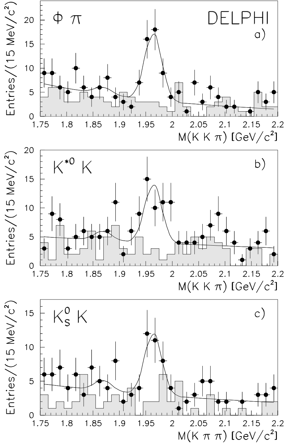
Figure 1: D_s \ell analysis: Invariant mass distributions for D_s^+ candidates, in the three analysed D_s^+ decay channels, accompanied by a lepton of opposite sign present in the same hemisphere and with p_t^{out} above 1.2 GeV/c. The “wrong-sign” combinations are given by the shaded histogram. The curves show the fit described in the text.
