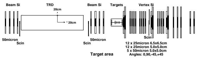
Figure 1: WA89 experimental set-up in 1993
