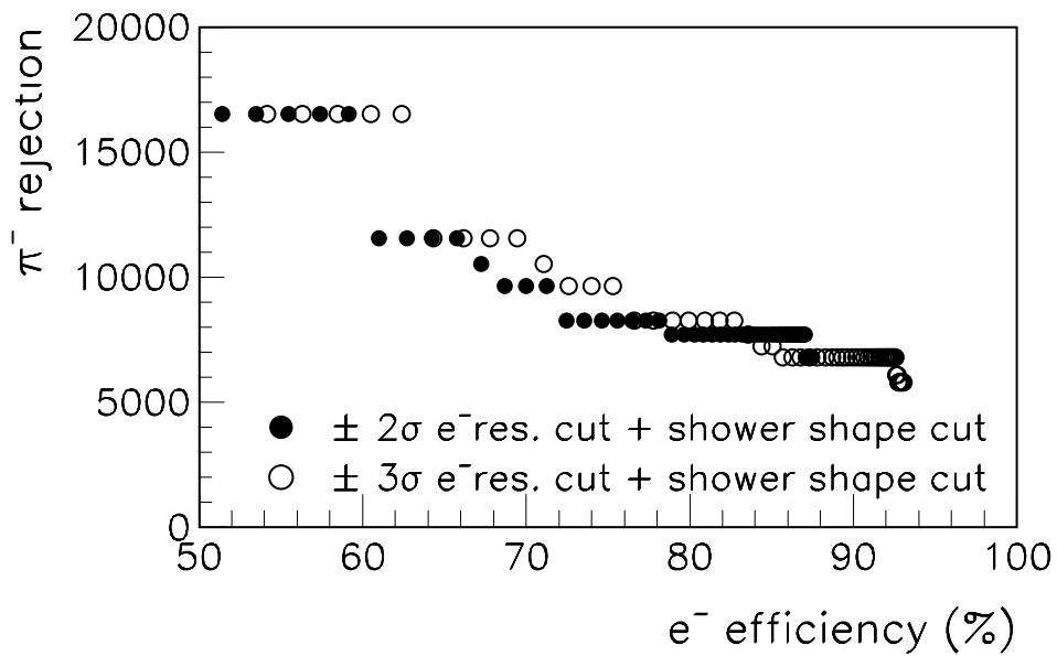
Fig. 15: Charged pion rejection factor as a function of electron efficiency at 80 GeV
