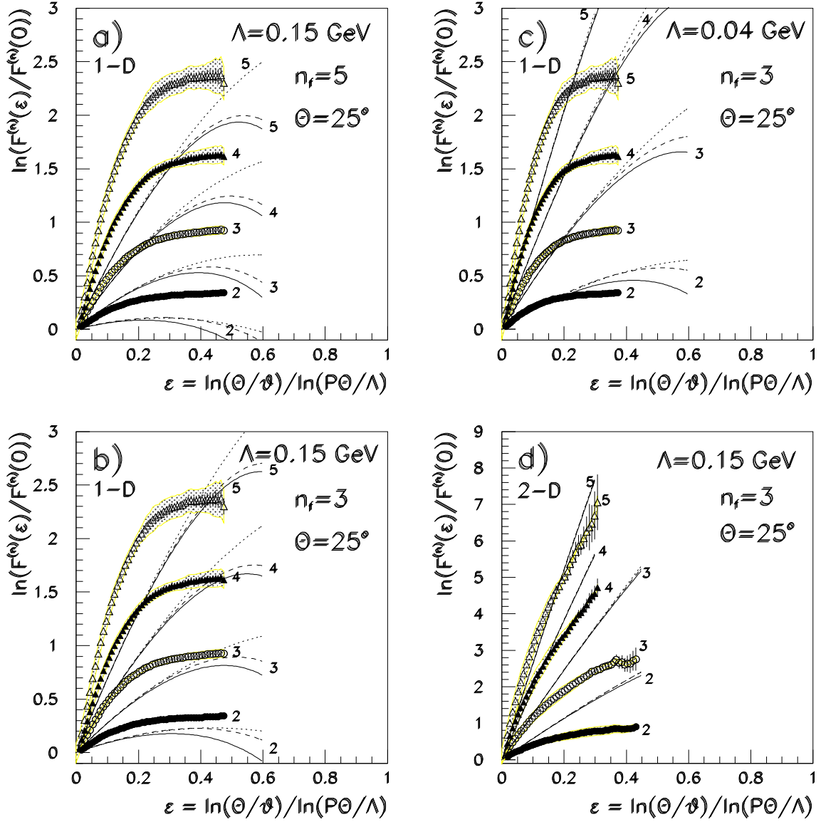
Figure 3: Factorial moments in 1-dimensional rings are compared with the analytical calculations of refs [4–6], eqs. 8 (solid lines), 11 (dashed lines), and 12 (dotted lines). The dependences on n_f and \Lambda are shown in a), b) and c). As a consistency test, 1- and 2-dimensional factorial moments are compared in b) and d) with same QCD parameters: note the different vertical scales. The orders 2 to 5 are indicated in all figures, the data are also distinguished by different symbols. The statistical errors are shown by the error bars, the shaded regions indicate the systematic errors. The 1-dimensional factorial moments agree very well with those measured by L3 [13].
