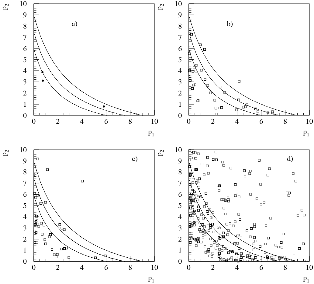
Figure 14: h\bar{q}q channel: distributions of the b-tagging variables of the two jets in the dijet opposite to the Z , as a function of each other, for (a) 172 GeV data, simulated (b) WW and (c) q\bar{q}(\gamma) events, and (d) simulated h\bar{q}q signal events with m_h = 70 \text{ GeV}/c^2 . The curves correspond to different values of k (2.0, 2.5 and 3.0 from lower to upper curve) in the last b-tagging requirement, as defined in the text. The normalisation of the simulated samples is arbitrary.
