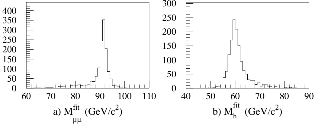
Figure 3: h\mu^+\mu^- channel: distributions of (a) the Z mass and of (b) the Higgs boson mass at the end of the analysis for simulated h\mu^+\mu^- events with m_h = 60 GeV/c 2 at 161 GeV.
