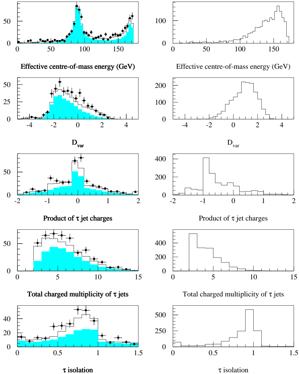
Figure 9: \tau^+\tau^- q\bar{q} channel: distributions of some analysis variables as described in the text. Plots on the left show a comparison between 172 GeV data and simulated background events (solid line) normalised to the experimental luminosity. The shaded area represents the contribution of the dominant q\bar{q}(\gamma) background. Plots on the right show the (unnormalised) expected distributions for a 70 \text{ GeV}/c^2 Higgs boson decaying into \tau^+\tau^- .
