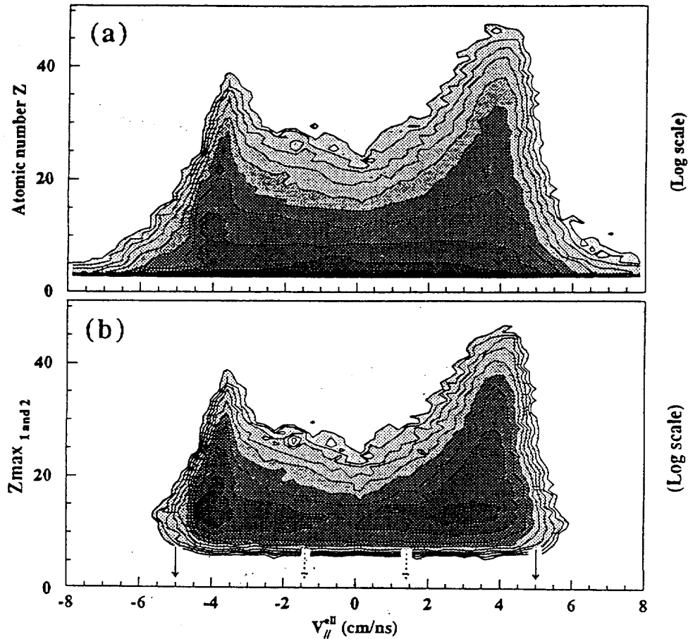
Figure 1: IMF V_{//} - Z plots for the Xe + Sn system at 50 MeV/u. In part (a) of the figure all IMF have been retained. In part (b), only the two heaviest of a given event are retained. Most events exhibit a two source behaviour and only few of them can be attributed to fusion. Extracted from ref 9.
