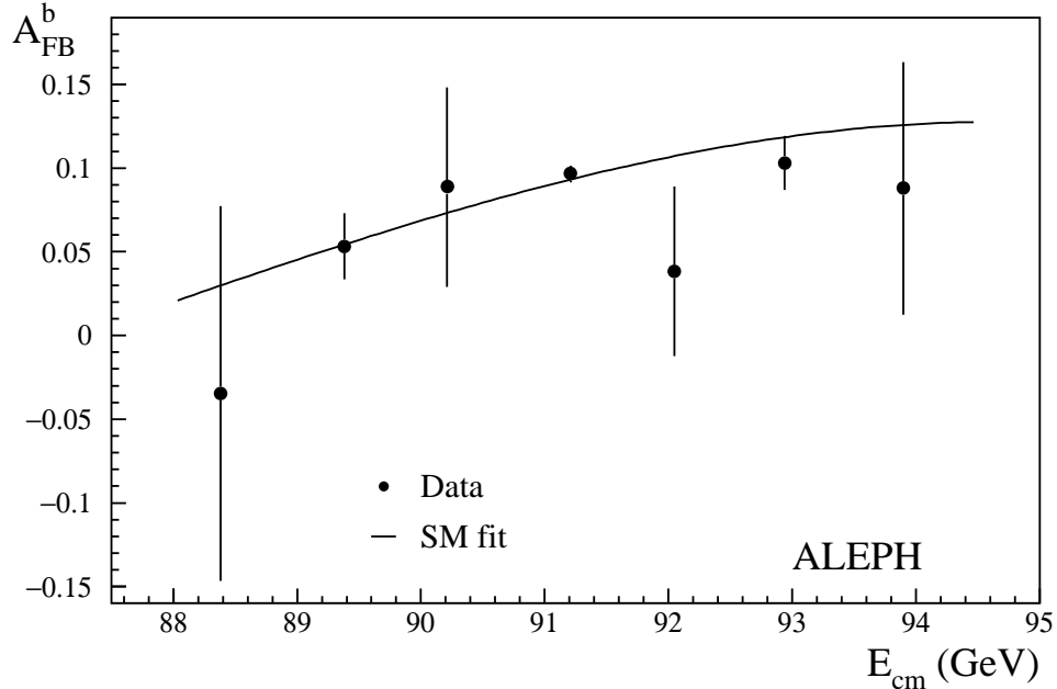
Figure 4: Extracted values of A_{\text{FB}}^b as a function of the centre-of-mass energy. The curve shows the Standard Model prediction fitted to the data used for the extraction of \sin^2\theta_{\text{W}}^{\text{eff}} .
