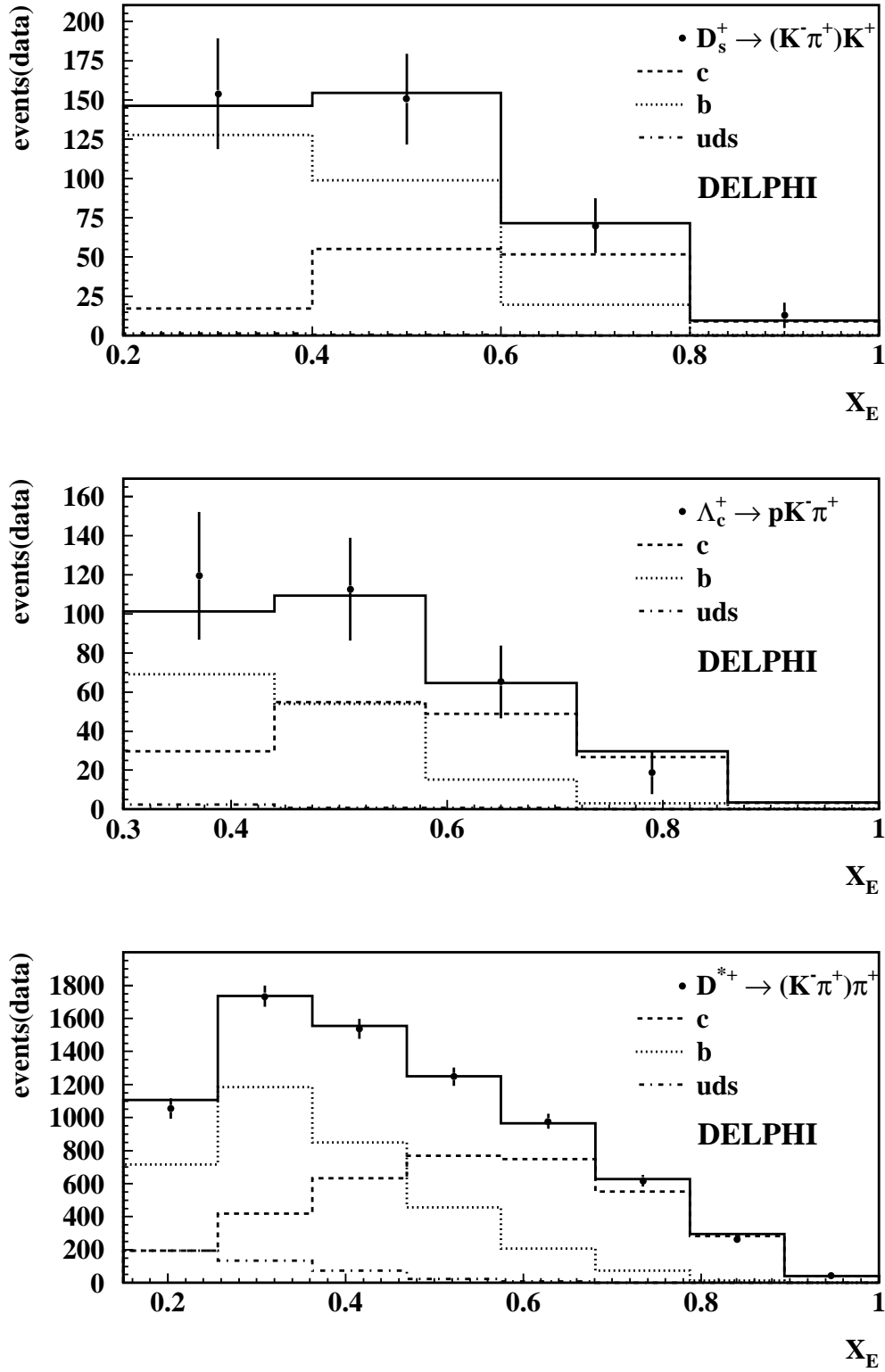
Figure 4: Background subtracted X_E spectra for the decays D_s^+ \rightarrow \bar{K}^*(892)K^+ (top), \Lambda_c^+ \rightarrow p \bar{K}^* \pi^+ and D^{*+} \rightarrow D^0 \pi^+ followed by D^0 \rightarrow K^- \pi^+ (bottom). The same conditions as in the caption of figure 3 are valid.
