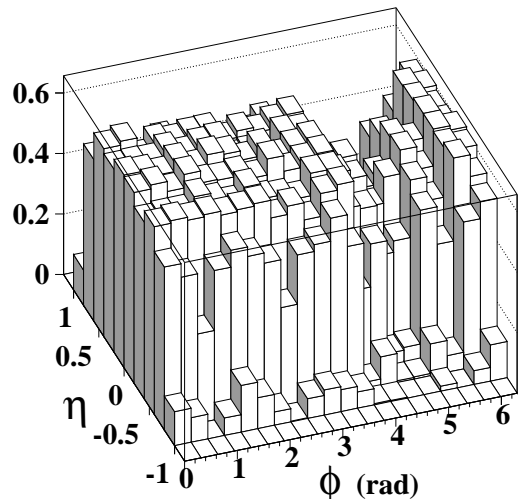
FIG. 2. The geometrical acceptance of the muon detector within the region |\eta| \leq 1 . \phi = \frac{3\pi}{2} is the downward ( -\hat{y} ) direction where the calorimeter support platform breaks into the muon system three-layer geometry.
