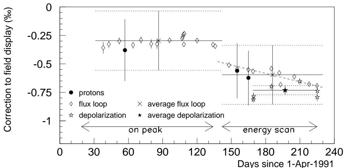
Figure 1: Beam energy calibrations in 1991. The measurements were corrected to the same temperature as mentioned in the text. Shown as a function of time is the correction to be applied to the energy obtained from measurements of the magnetic field in the reference magnet. The individual flux loop measurements are shown with the error from the temperature correction only; the full error is shown by the horizontal dotted lines representing the average of all measurements before and during the energy scan, respectively. The error bar drawn on the average of the depolarization points represents the r.m.s. spread of the individual measurements.
