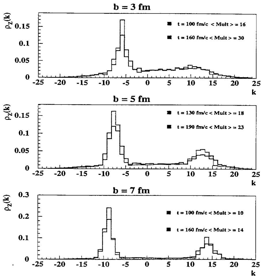
Figure 6: Charged density distributions for different impact parameters: the predictions of a BNV simulation are shown for different asymptotic times and the corresponding mean charged particle multiplicities ( \text{Mult} ) are indicated.
