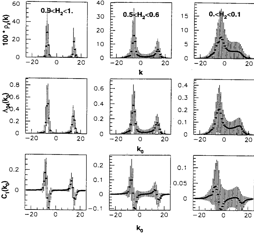
Figure 4: The first row presents the charge density distributions for three H_2 bins, the second row shows the \Lambda_{04}(k_0) distributions and the third row presents C_1(k_0) distributions.
