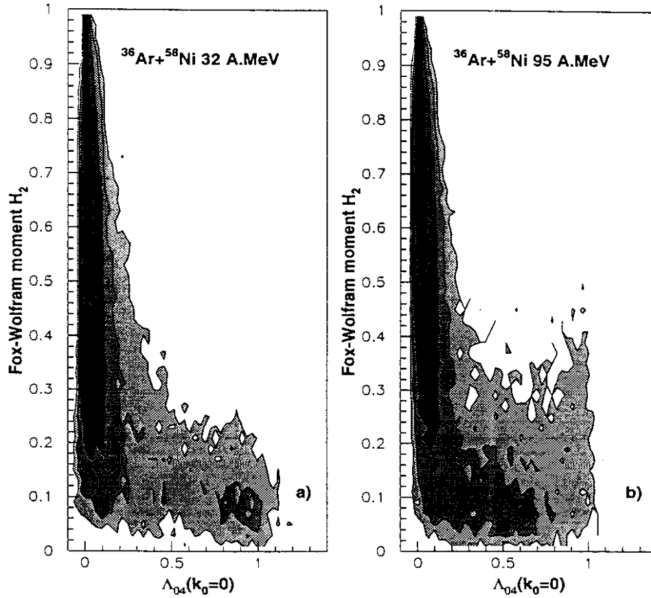
Figure 3: The correlation between H_2 and \Lambda_{04}(k_0 = 0) is shown for beam energies of 32 and 95 A.MeV. The isocontours are in logarithmic scale.
