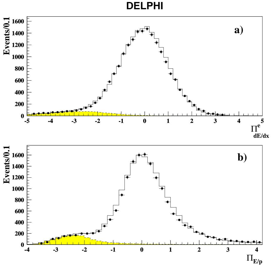
Figure 1: Distribution of electron identification variables for electron test samples: a) pull dE/dx and b) pull E/p for electron hypothesis. The solid line is for all simulation, the hatched area represents the background (anything except \tau decays to electrons) and the circles are the data.
