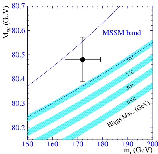
FIG. 61. A comparison of the W boson and top quark mass measurements by the D\bar{O} collaboration with the standard model predictions for different Higgs boson masses [56]. The width of the bands for each Higgs boson mass value indicates the uncertainty due to the error in \alpha(M_Z^2) . Also shown is the range allowed by the MSSM [22].
