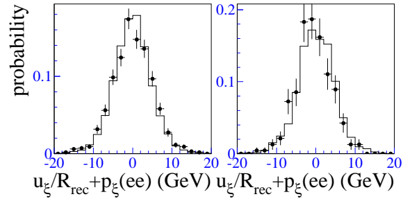
FIG. 32. The \xi -balance distribution for the Z boson data ( \bullet ) and the fast Monte Carlo simulation ( \text{—} ). The plot on the left is for the CC/CC + CC/EC Z events and the plot on the right is for the EC/EC Z events.
