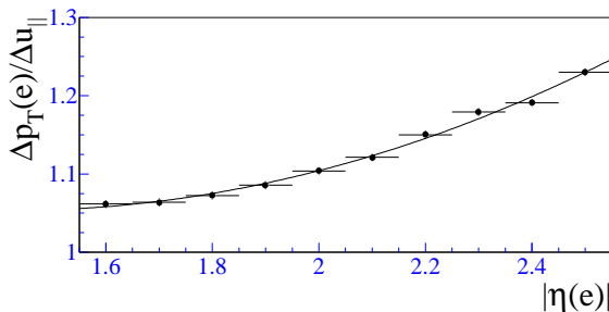
FIG. 23. The ratio of the \langle\Delta u_{||}/\delta\eta\delta\phi\rangle corrections to the electron and the recoil as a function of electron \eta .
