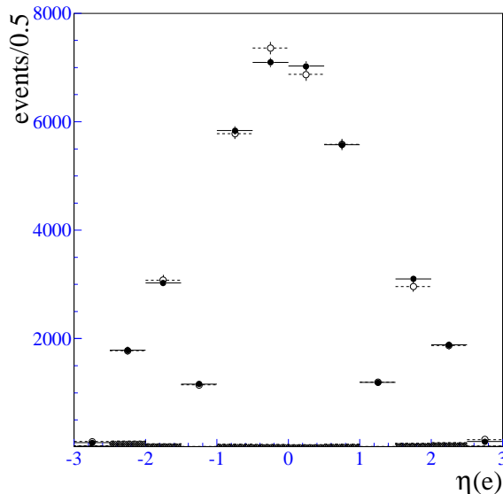
FIG. 38. \eta distribution of the electron from W \rightarrow e\nu decays from background-subtracted data ( \bullet ), efficiency-corrected Monte Carlo ( \circ ) and the jet background (shaded histogram). The distributions drop near |\eta|=1.2 because there is no EM calorimetry in the range 1.1 < |\eta_{\text{det}}| < 1.4 .
