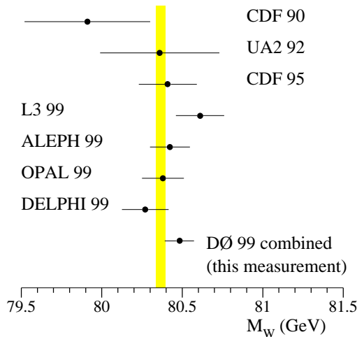
FIG. 60. A comparison of this measurement with previously published W boson mass measurements (Table XI). The shaded region indicates the predicted W boson mass value from global fits to the Z boson lineshape data [11].
