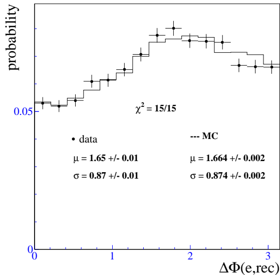
FIG. 36. The azimuthal difference between electron and recoil directions for the W data ( \bullet ) and the Monte Carlo simulation (—). The mean ( \mu ) and r.m.s. ( \sigma ) of the distributions and the \chi^2 is also shown.
