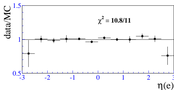
FIG. 39. The ratio of the background-subtracted data and efficiency-corrected Monte Carlo. The Monte Carlo has been normalized to the data. The \chi^2 is with respect to unity.
