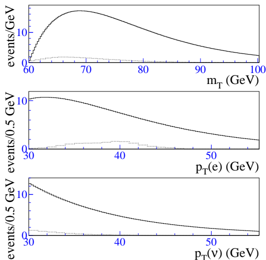
FIG. 42. Shapes of m_T , p_T(e) , and p_T(\nu) spectra from hadron (—) and Z boson (- - -) backgrounds with the proper relative normalization.
