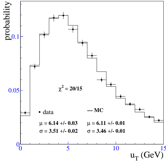
FIG. 35. The recoil momentum ( u_T ) spectrum for the W data ( \bullet ) and the Monte Carlo simulation ( \text{---} ). The mean ( \mu ) and r.m.s. ( \sigma ) of the distributions and the \chi^2 is also shown.
