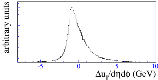
FIG. 22. The distribution of \Delta u_{||}/\delta\eta\delta\phi in the W signal sample, corrected to \mathcal{L}=0 , |\eta|=2 , u_{||}=0 .
