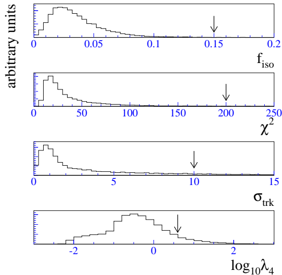
FIG. 13. Distributions of the EC electron identification variables for W \rightarrow e\nu candidates. The arrows indicate the cut values.
