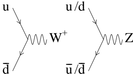
FIG. 2. Lowest order diagrams for W and Z boson production.
