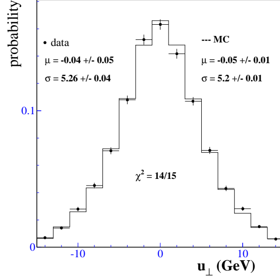
FIG. 34. The u_{\perp} spectrum for the W data ( \bullet ) and the Monte Carlo simulation ( \text{---} ). The mean ( \mu ) and r.m.s. ( \sigma ) of the distributions and the \chi^2 is also shown.
