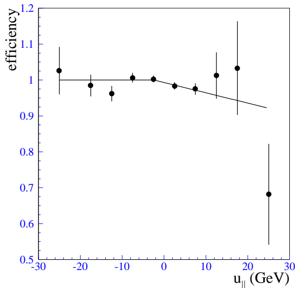
FIG. 24. The EC electron selection efficiency as a function of u_{\parallel} .
