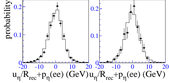
FIG. 31. The \eta -balance distribution for the Z boson data ( \bullet ) and the fast Monte Carlo simulation ( \text{—} ). The plot on the left is for the CC/CC + CC/EC Z events and the plot on the right is for the EC/EC Z events.
