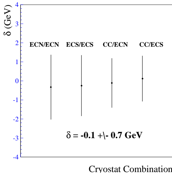
FIG. 25. The ECCEM offset measurements using the CC/EC and EC/EC Z samples.
