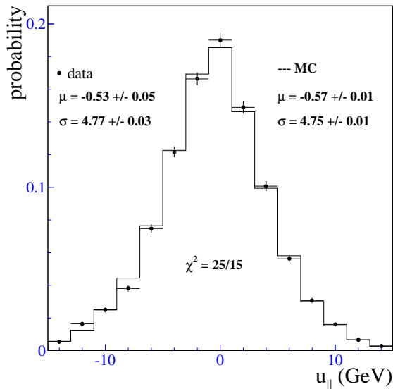
FIG. 33. The u_{\parallel} spectrum for the W data ( \bullet ) and the Monte Carlo simulation (—). The mean ( \mu ) and r.m.s. ( \sigma ) of the distributions and the \chi^2 is also shown.
