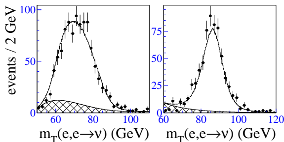
FIG. 59. Spectra of the Z boson transverse mass, from the CC/EC data (left) and the EC/EC data (right). The superimposed curves show the maximum likelihood fits and the shaded regions show the estimated backgrounds.
