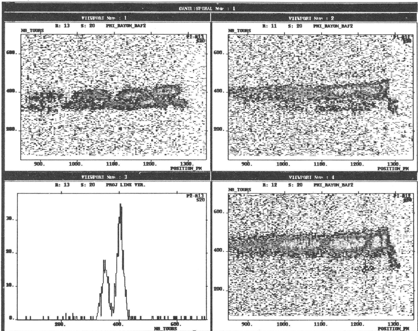
Figure 2: Examples of spectra obtained by scanning the radial probe. The total phase width of the beam is around 25^\circ . These spectra were taken for different RF voltages. At the lower left corner, an example of a projection in the top left spectrum, is shown. The display of such a slice is possible at any probe location.
