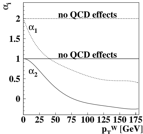
FIG. 1. The angular parameters \alpha_1 (dashed) and \alpha_2 (solid) as functions of p_T^W . These parameters are evaluated integrated over the W boson rapidity, y . In the absence of QCD effects \alpha_1 and \alpha_2 equal 2.0 and 1.0, respectively.
