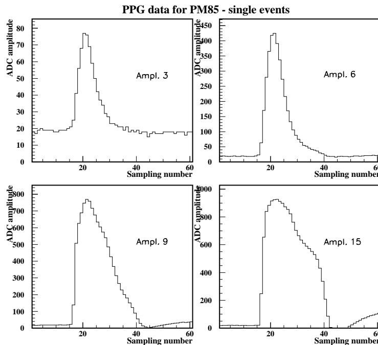
Figure 3: Example of four single charge injection events. Amplitude 3 is in the first linear region; amplitude 6 peaks at the first “knee”, 9 at the second and 15 in the third region. Note the different scales.
