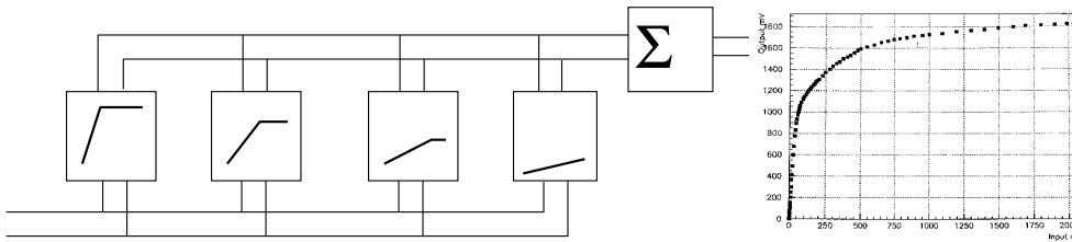
Figure 2: Concept of the compressor. This circuitry forms a sum of the outputs from four linear amplifiers with gains approximately 18.5, 1.3, 0.14 and 0.09 and upper cutoffs on the input voltage of 60, 470 and 1200 mV respectively. The fourth amplifier spans the full 2000 mV input range of the compressor. To the right, a typical transfer function as measured in the laboratory.
