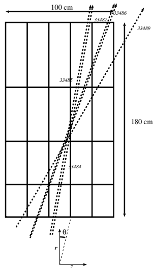
Figure 7: Impact points and direction of the beam in the five runs considered in this analysis.
