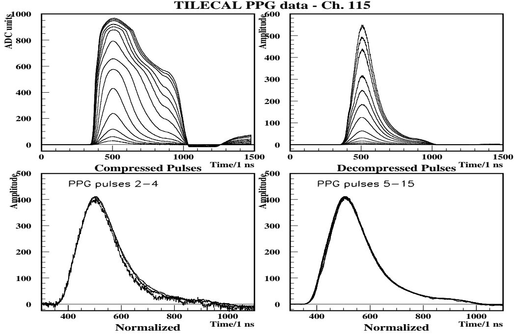
Figure 10: Reconstructed pulse shapes. Compressed (top left) and decompressed (top right). The decompressed pulses are normalized to their peak values (bottom). Due to noise, the peak value is not sharply defined for low amplitudes, thus the discrepancy between the curves in the lower left plot.
