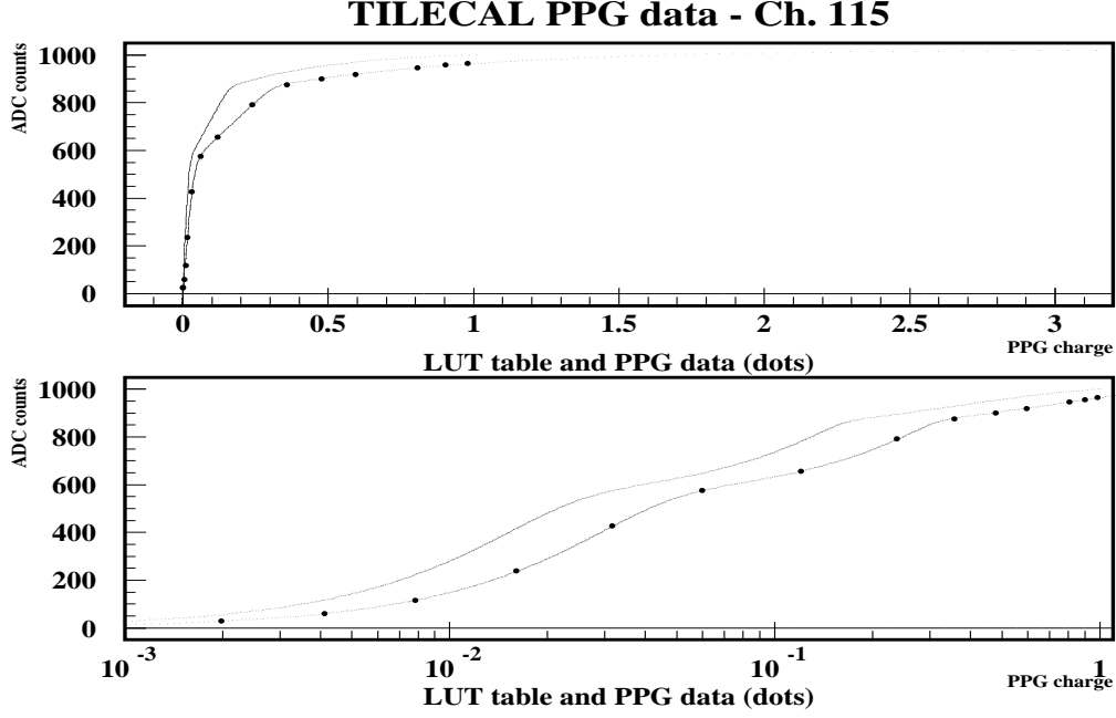
Figure 11: Model LUT (higher curve) compared to stretched LUT (lower curve) from three parameter fit in linear (top) and logarithmic scale (below). PPG pulses are shown as fat dots.
