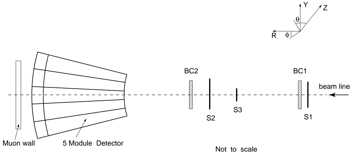
Figure 5: Test beam layout for the 1995 standalone test beam.
