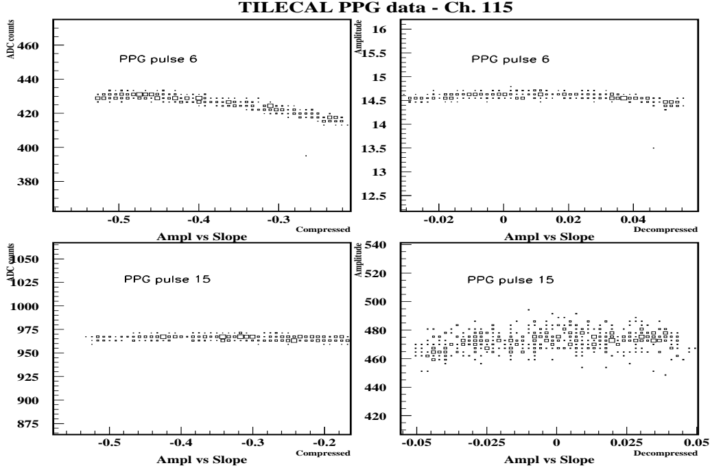
Figure 9: Peak amplitude versus slope (phase estimator) for compressed (left, in ADC counts) and decompressed (right, in pC) PPG pulses 6 (top) and 15 (bottom).
