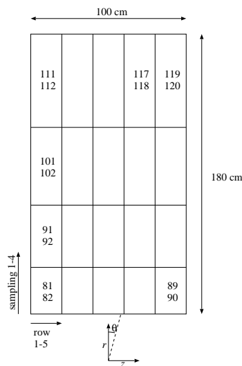
Figure 4: Cell layout and dimensions of a 1 m Tilecal prototype module. Numbers refer to the PMT (channel) numbers of the central module.
