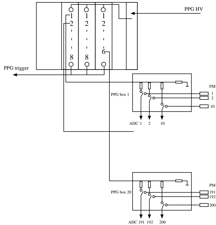
Figure 6: Layout of the PPG system.
