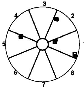
Figure 4: Cross section of the eight-fold segmented Ge detector shown in fig. 2. The simulated interaction points are indicated by full circles and the identified interaction points by open squares.
