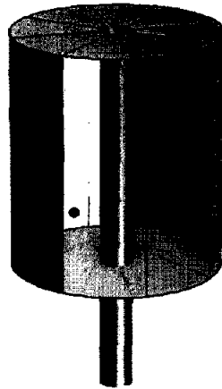
Figure 2: Eight-fold segmented true-coaxial Ge detector with four simulated interactions of \gamma -radiation with the detector shown as full circles.
