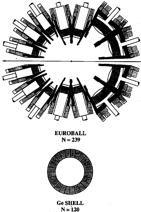
Figure 1: Cross-sections of the \gamma -ray array EUROBALL and a Ge shell. The two spectrometers are drawn approximately to scale. The Ge detectors are shown in grey and the BGO anti-Compton shields in black.
