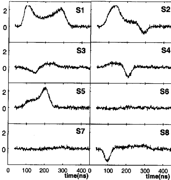
Figure 3: Simulated pulse shapes of preamplified signals derived from the eight segments corresponding to the simulated interaction points in the Ge detector shown in fig. 2.
