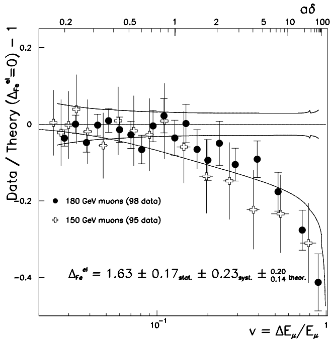
Fig. 7. Determination of \Delta_{Fe}^{el} , the elastic nuclear form factor correction to muon bremsstrahlung. The data (full circles) are compared with theoretical predictions with \Delta_{Fe}^{el}=0 (horizontal line at 0) and the fit to the data with \Delta_{Fe}^{el}=1.63 shown by the curve. The effect of systematic errors is shown by the two curves around zero. For comparison, the data of [14] are plotted by crosses. The error bars are the quadratic sum of statistical and systematic errors. The upper horizontal scale is in units of the product of the Bohr radius of the iron atom ( a ) and the minimal momentum transfer to the iron nucleus ( \delta ). The values of a\delta determine the regions of screening ( a\delta \leq 1 ) and of no screening ( a\delta \geq 1 ) of the nucleus by atomic electrons
