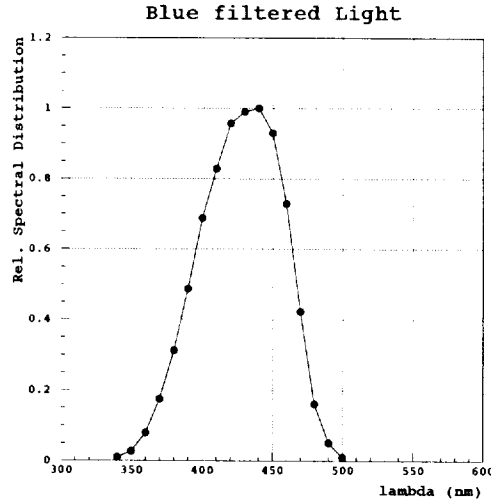
Figure 21 : Relative spectral irradiance from a tungsten lamp operated at a color temperature of 2856 K, and transmitted by a "blue" filter Filter corrected spectral (Corning Cs No. 5-58 polished to half stock thickness).
