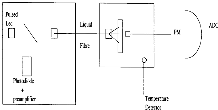
Figure 45 : Experimental set-up used for the test of the temperature effect on the PMT amplification. The PMT box temperature is regulated within 1^\circ C, and is recorded for each event for the offline analysis.
