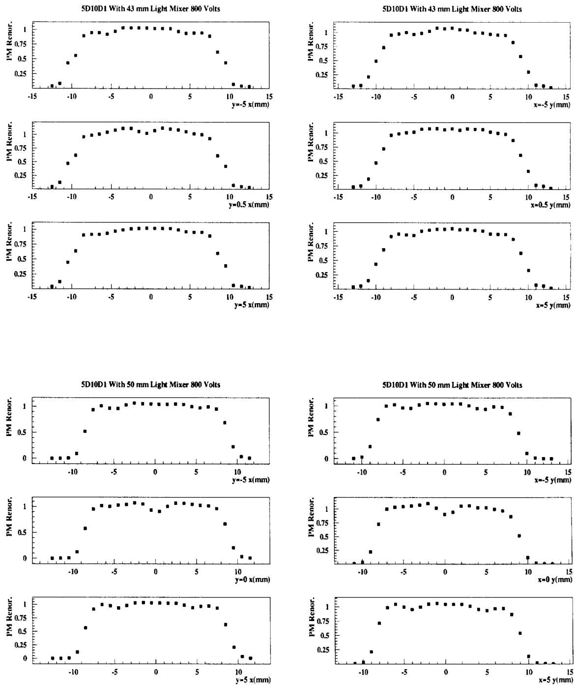
Figure 34-b : Same as on Figure (34-a). The length of the "light mixer" was 43 mm (top) and 50 mm (bottom).
