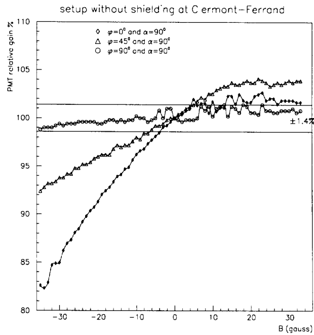
Figure 68 : Effect of the magnetic fields on a bare R5900 PMT: a) and b) Field perpendicular to the z-axis ( \alpha = 90^\circ ) with various \varphi angles, in the B ranges of about (0, 200 gauss) and ( \pm 35 gauss), respectively.
