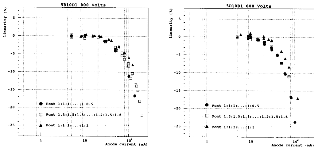
Figure 54 : R5900 linearity (PMT # 5D10D1 of the second generation), as a function of the anode current for three different voltage repartitions: open squares correspond to the 1.5:1.5:1.5:1:....:1.2:1.5:1.8 configuration, full circles to the 1:1:1:....:1:1:0.5 configuration, and full triangles to the 1:1:1:....:1:1 configuration. On left part, PMT voltage was set to 800 Volts, on right part to 600 Volts.
