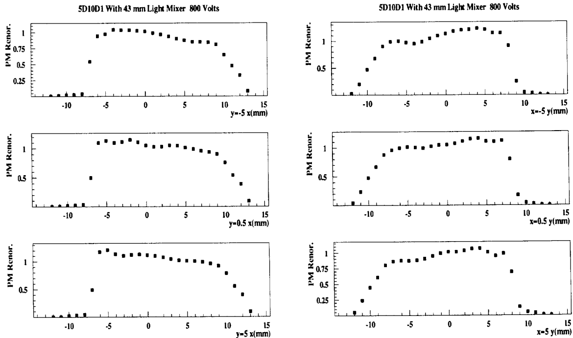
Figure 35 : Variation of the PMT (#5D10D1) response, as a function of x and y coordinate of a 1 \times 1 \text{ mm}^2 illuminated window of this PMT photocathode moving in front of the output face of the light mixer (the PMT is simply used as a spot photodetector). The signal of that spot photodetector, after pedestal subtraction is renormalised to the averaged response on a 16 \times 16 \text{ mm}^2 central square window on the output face of the "light mixer". The length of the "light mixer" was 43 mm, and the fiber points to the top left corner on the "light mixer" input face.
