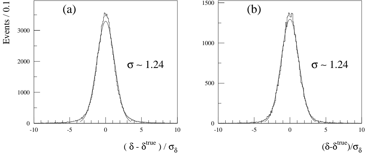
Figure 6: Pull distribution (\delta - \delta^{\text{true}})/\sigma_{\delta}^{\text{Tracking}} in Monte Carlo (a) 1-1 sample (b) 1-3 sample. \delta is the reconstructed 3DIP; \delta^{\text{true}} is defined as \delta\vec{C}_0^{\text{true}} \cdot \hat{H} , where \delta\vec{C}_0^{\text{true}} is computed at generation level and \hat{H} is the reconstructed projection direction.
