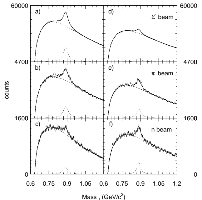
Fig. 2a-f. K_{890}^0 \pi^\pm effective mass distributions: K_{890}^0 \pi^- (a - c); K_{890}^0 \pi^+ (d - f)
