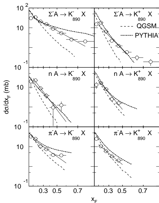
Fig. 5. Comparison of the measured differential cross sections with PYTHIA and QGSM predictions. The solid line shows the fit of experimental data by (1)
