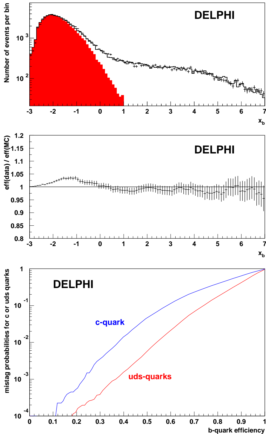
Figure 1: b-tagging: Top: distributions of the combined b-tagging variable x_b , in 1999 Z data (dots) and simulation (histogram). The contribution of udsc-quarks is shown as the dark histogram. Middle: ratio of integrated tagging rates in Z data and simulation as a function of the cut in x_b . Bottom: mistag probabilities for c or uds-quarks as a function of the efficiency for b-quarks, estimated from simulated Z data.
