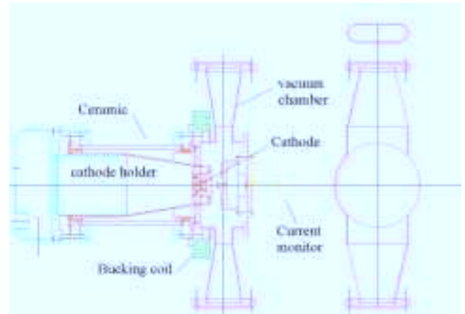
Fig.1 Mechanical scheme of CLIO GUN
