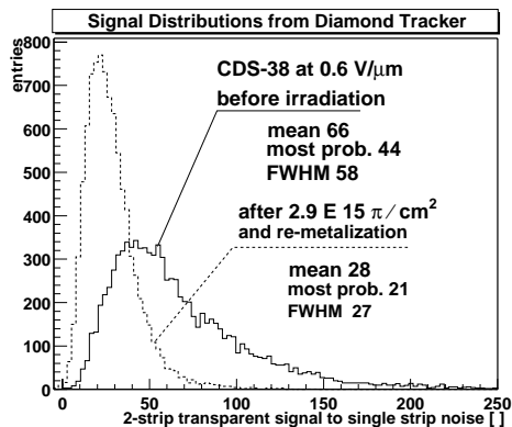
Fig. 6. Transparent 2-strip charge signal-to-noise distributions before (solid line), after pion irradiation with 2.9 \times 10^{15} \pi/\text{cm}^2 (dashed line).
