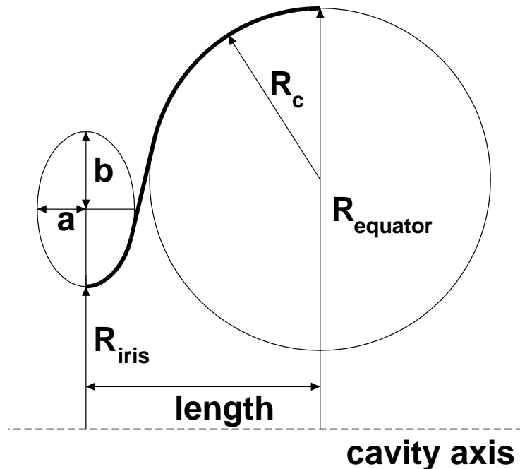
Figure 6: Contour of a half cell.
