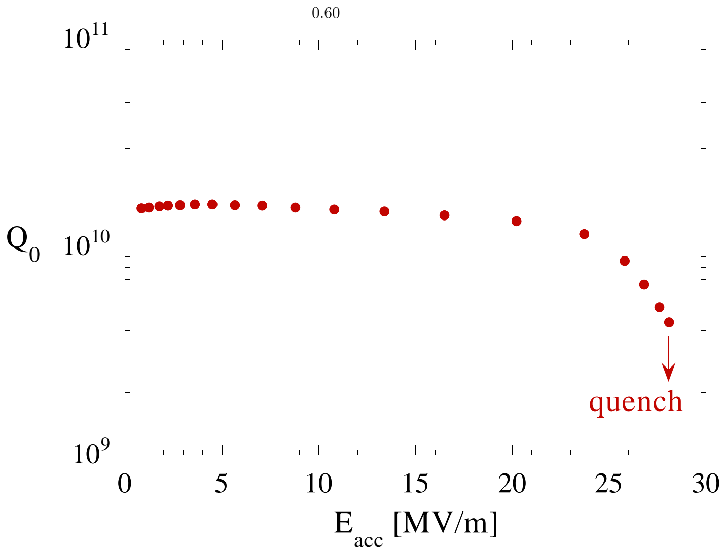
Figure 30: Excitation curve of a TESLA 9-cell cavity showing a drop of quality factor without any field emission.
