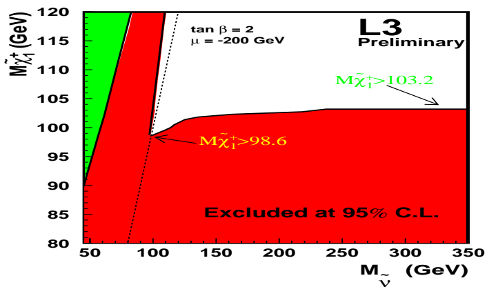
Figure 5. Excluded region in (M_{\tilde{\chi}_1^\pm}, M_{\tilde{\nu}} ) plane for \tan\beta = 2 and \mu = -200 GeV. The lowest mass limit is set from charginos and slepton searches
