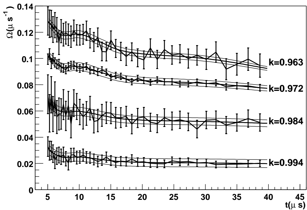
Fig. 7. \Omega_{k_{\text{eff}}^{\text{D}}}(t) fits for 4 reactors of different k_{\text{eff}}^{\text{D}} , after weighting P(\tau) by the importance
