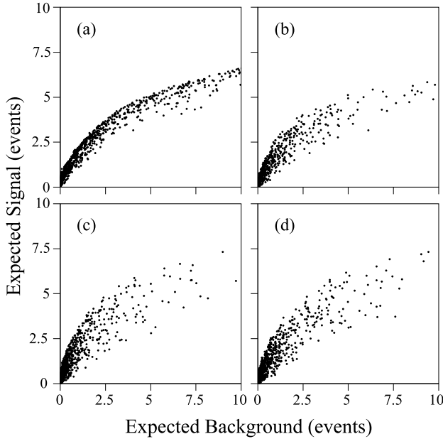
FIG. 15. Results of the random grid search in terms of expected signal vs expected background for the e +jets topological analysis for four possible variable sets: (a) \mathcal{A}(W + \text{jets}) and h , (b) \mathcal{A}(W + \text{jets}) , h , and \cancel{E}_T , (c) \mathcal{A}(W + \text{jets}) , H_T , and \cancel{E}_T , (d) \mathcal{A}(W + \text{jets}) , H_T , and p_T(W) . See text for definitions of these variables.
