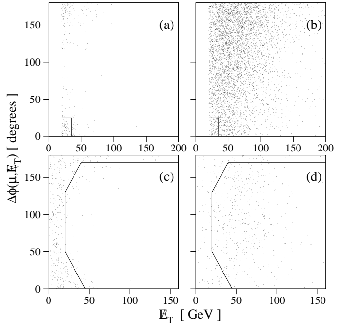
FIG. 21. Scatter plots of \Delta\phi(\mu, \cancel{E}_T) vs \cancel{E}_T for (a) e +jets/ \mu QCD multijet background, (b) t\bar{t} \rightarrow e +jets/ \mu , (c) \mu +jets/ \mu QCD multijet background, and (d) t\bar{t} \rightarrow \mu +jets/ \mu . The solid lines define the cut boundaries.
