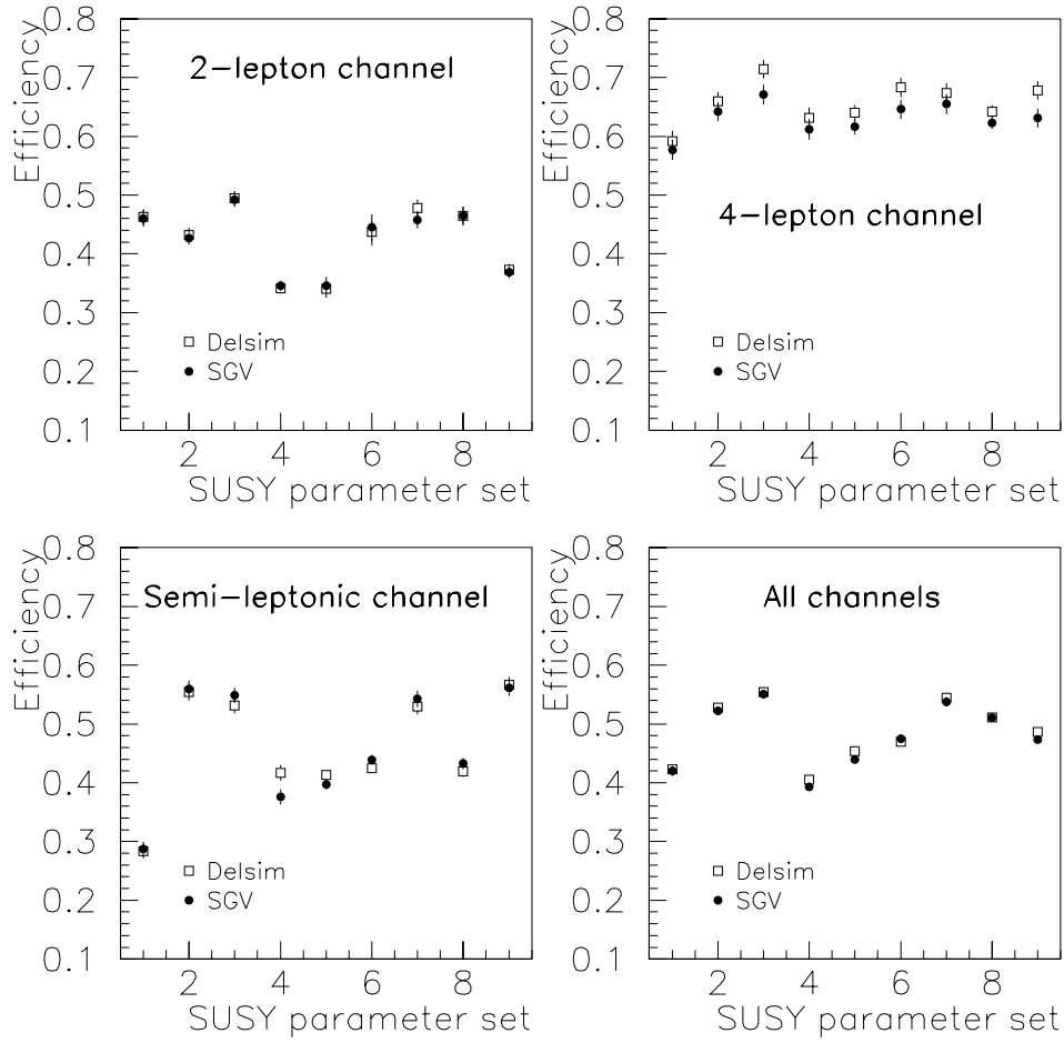
Figure 4: SGV-DELSIM comparison for nine SUSY parameter sets with different sneutrino masses and total widths (see Table 2) in the case of a \lambda_{121} coupling and for \tan\beta = 1.5 , \sqrt{s} = 206.5 GeV. For this comparison, the same number of events was simulated with SGV and DELSIM.
